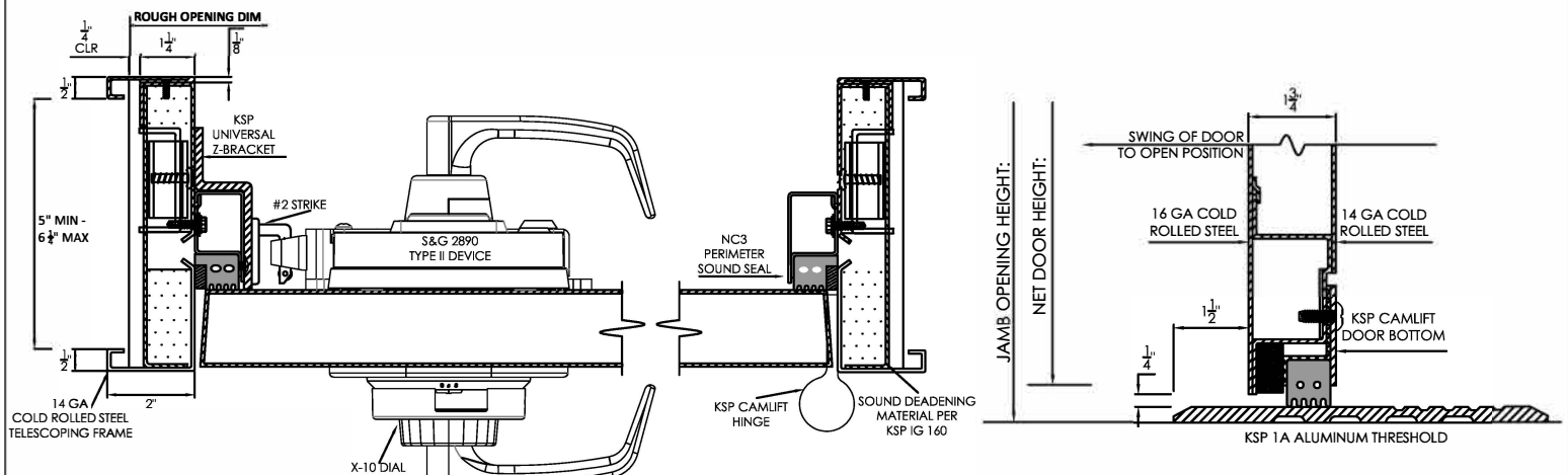
HORIZONTAL SECTION
