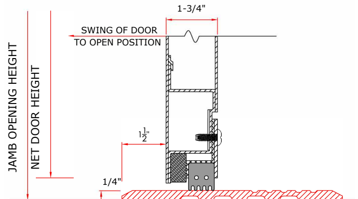
VERTICAL SECTION
