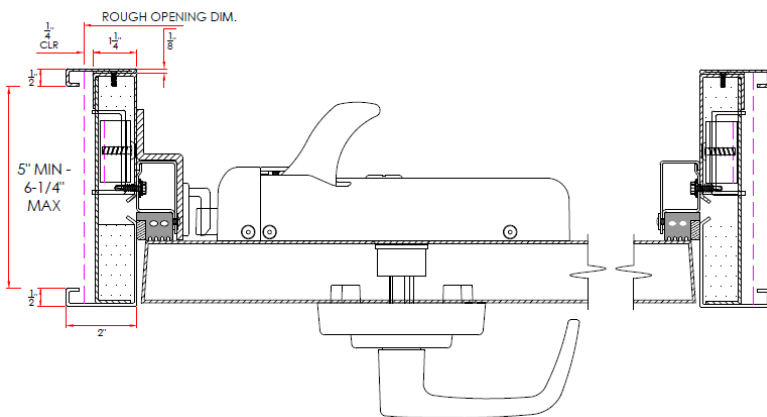
HORIZONTAL SECTION
