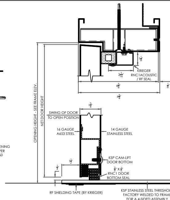
VERTICAL SECTION
