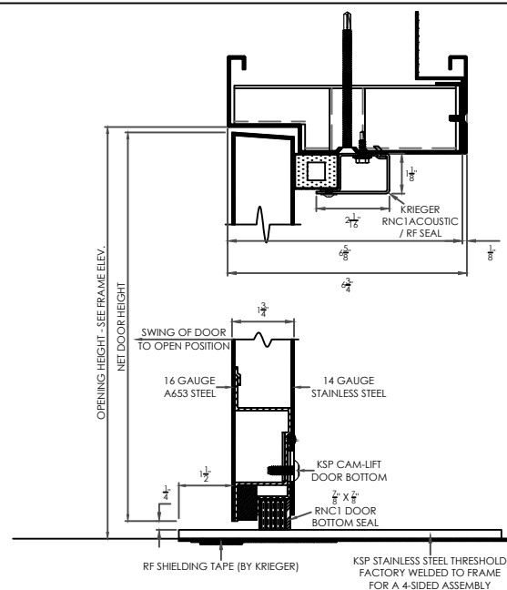
VERTICAL SECTION
