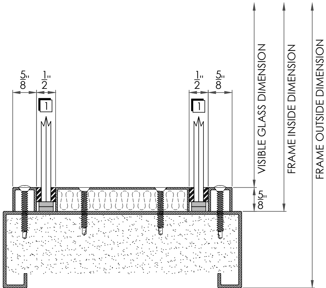
1 1/4" LAMINATED GLASS
