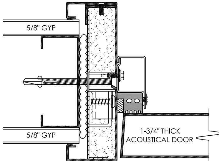
FINISHED FRAME
