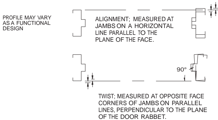
FIGURE 5 Installation Tolerances
